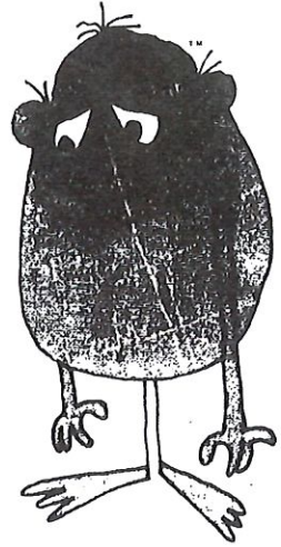
"OGRE-EDITOR"
